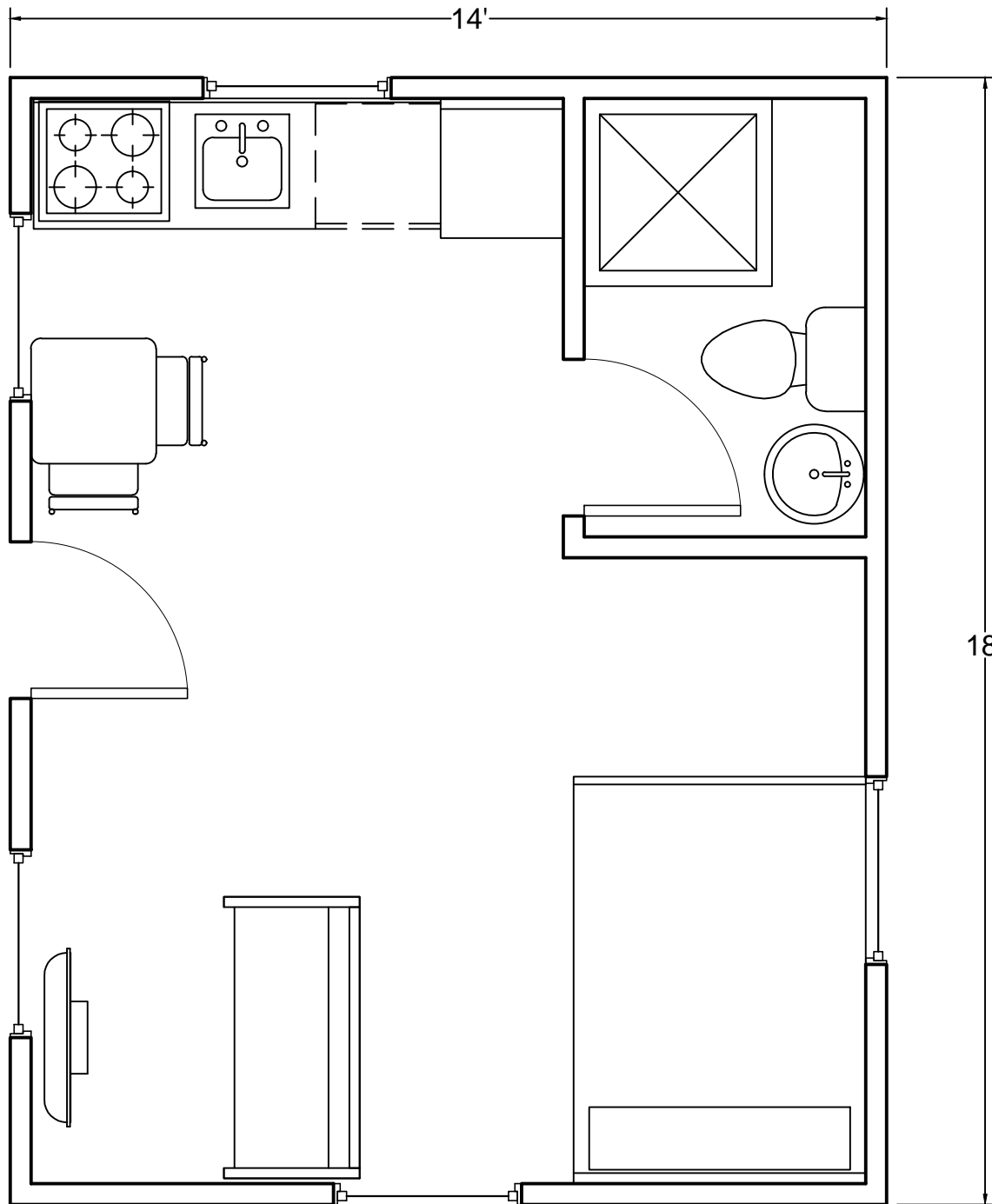
MHUD PMCU Starter House Plan Floor Plan: One Bedroom 14'x18' Scale: \frac{3}{8} " = 1'-0"
